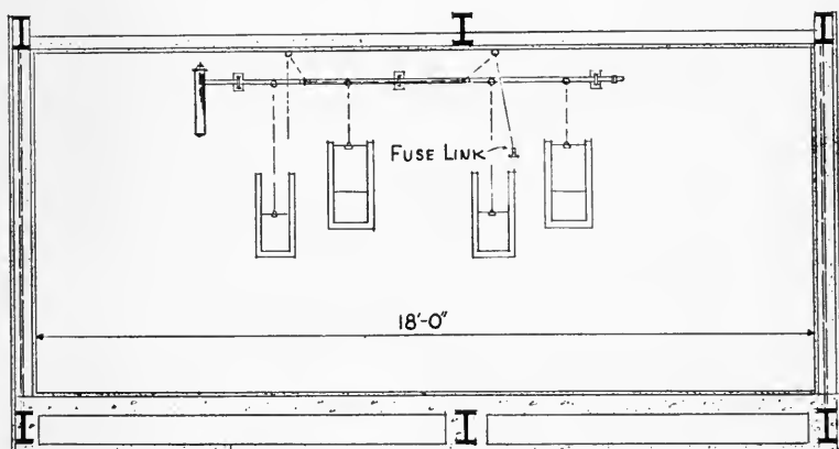
FIG. 4. Front elevation of projection booth.
